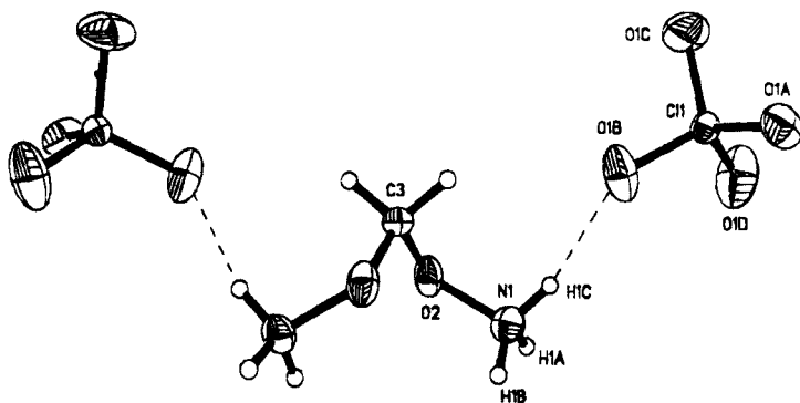
Figure 1. An ORTEP plot of the full diperchlorate salt unit. The asymmetric unit is just the labeled atoms above, \frac{1}{2} of the full salt. A crystallographic two-fold symmetry axis bisects the cation; it is a vertical axis in this view. 60
